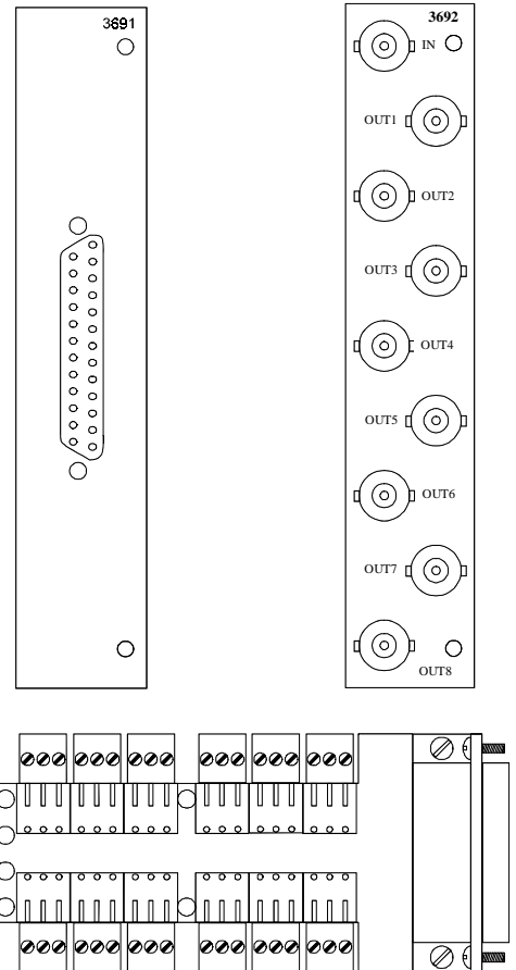
3990 D type to removable screw terminal adapter
